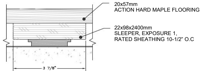
ActionProAir_NR_WBS Section across room length
