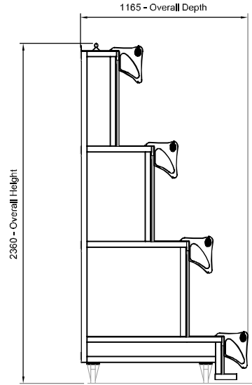
SIDE ELEVATION (Unit in Store Position)
