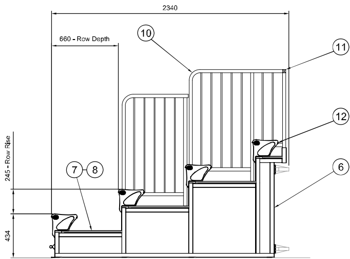
SIDE ELEVATION - Maxam 24 (HSM24)
